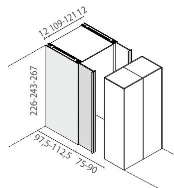
c. Double Kabin Mechanism facing the inner opening
